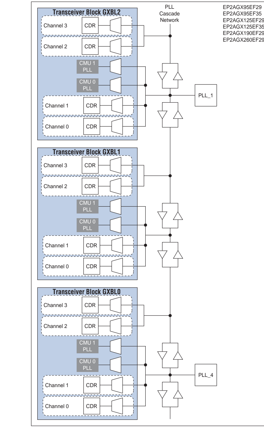
Figure 2-33. FPGA Fabric PLLs Transceiver PLLs Cascading Option Allowed in the EP2AGX95EF29, EP2AGX95EF35, EP2AGX125EF29, EP2AGX125EF35, EP2AGX190EF29, and EP2AGX260EF29 Devices
