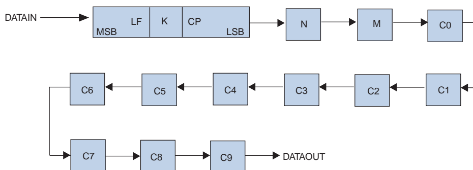
Figure 5-42. Scan Chain Order of PLL Components for Top and Bottom of Arria II GZ PLLs (Note 1)
