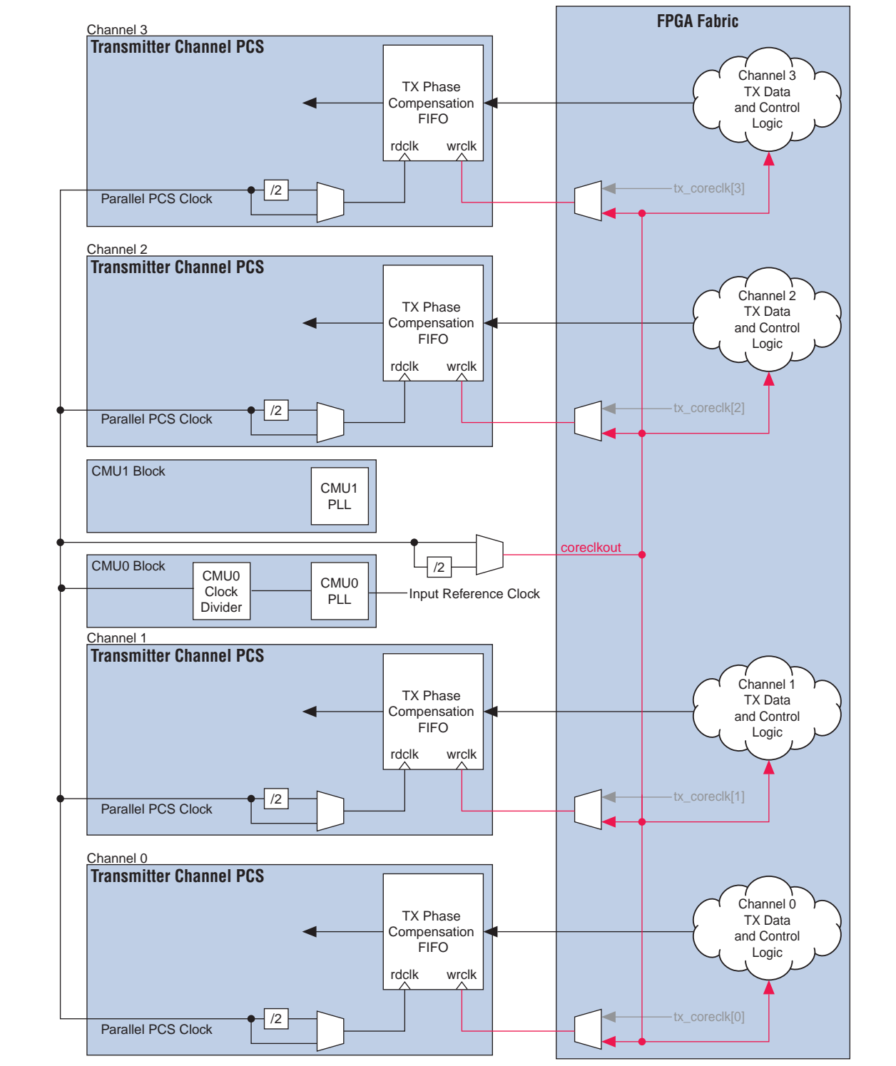
Figure 2-20. FPGA Fabric-Transmitter Interface Clocking in an x4 Bonded Channel Configuration
