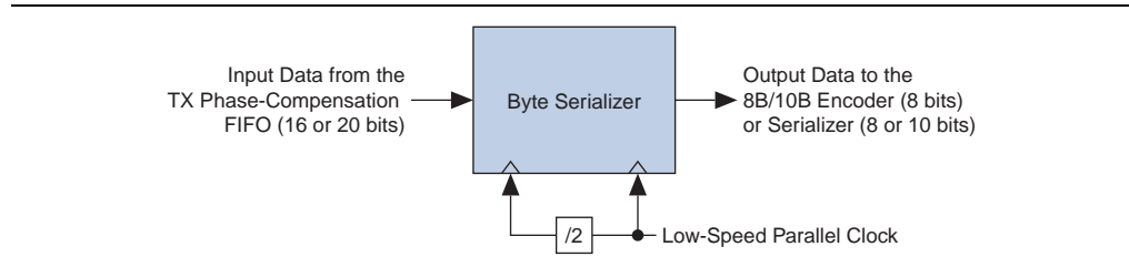
Figure 1–13. Byte Serializer Datapath for Arria II GX Devices
