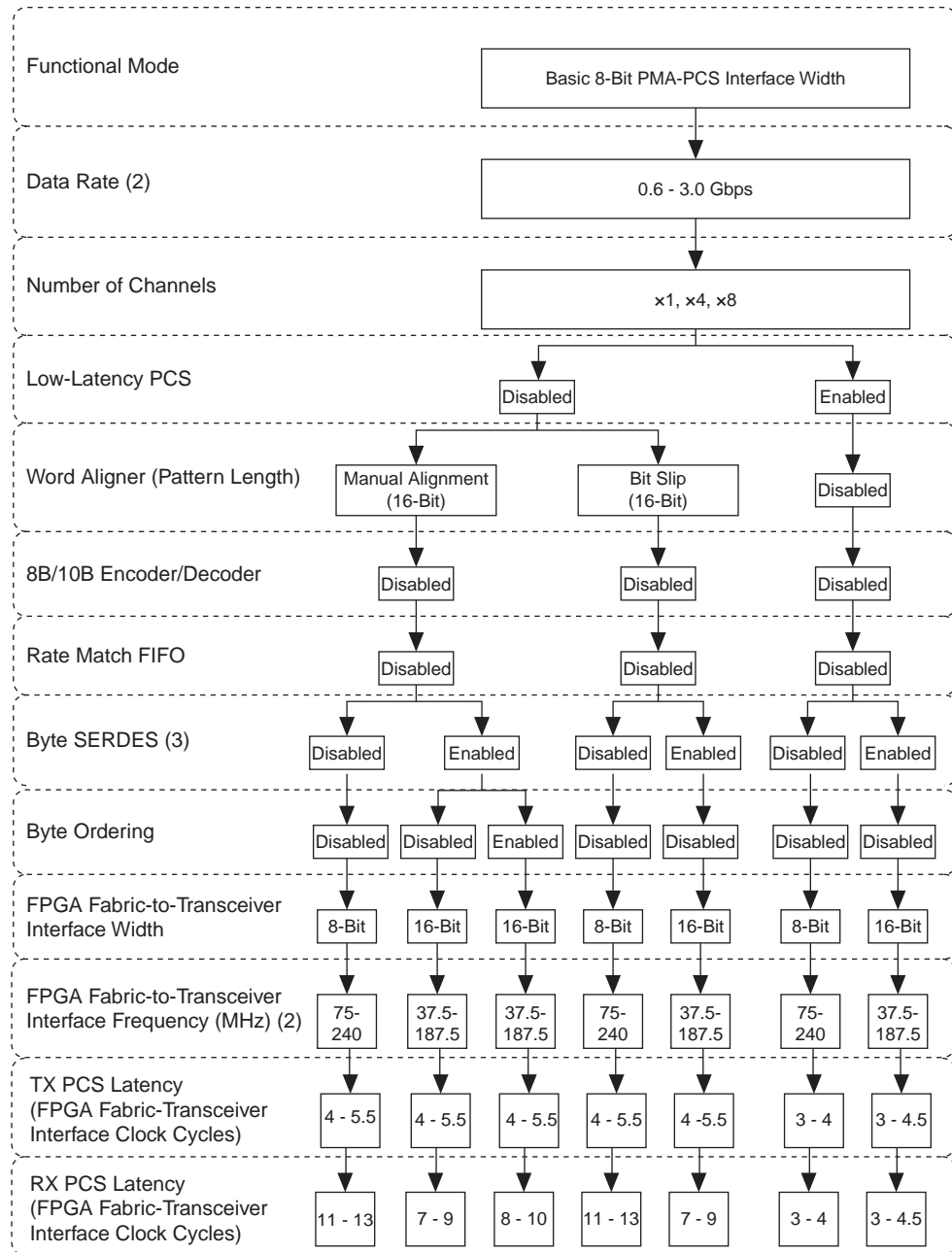
Figure 1-51. Transceiver Configurations in Basic Mode with an 8-Bit Wide PMA-to-PCS Interface (Note 1)
