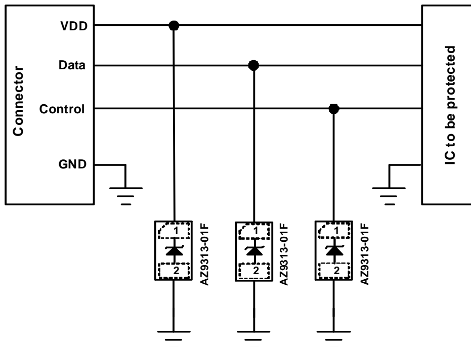
Fig. 1 ESD protection scheme by using AZ9313-01F.
