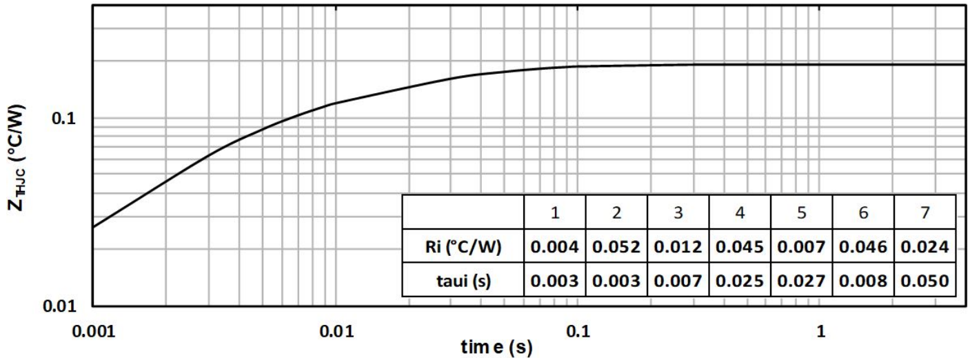
Figure 1-15. Maximum Thermal Impedance
