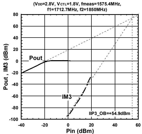
Out-of-band IIP3
