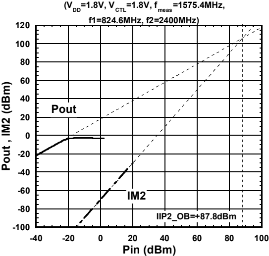
Out-of-band IIP2
