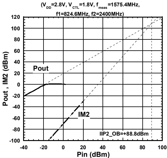
Out-of-band IIP2
